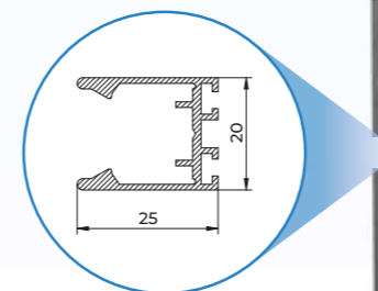
STARTING/ARRIVING CHANNEL Weight gr/mt: 308*
