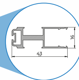
HANDLE BAR Weight gr/mt: 471*
